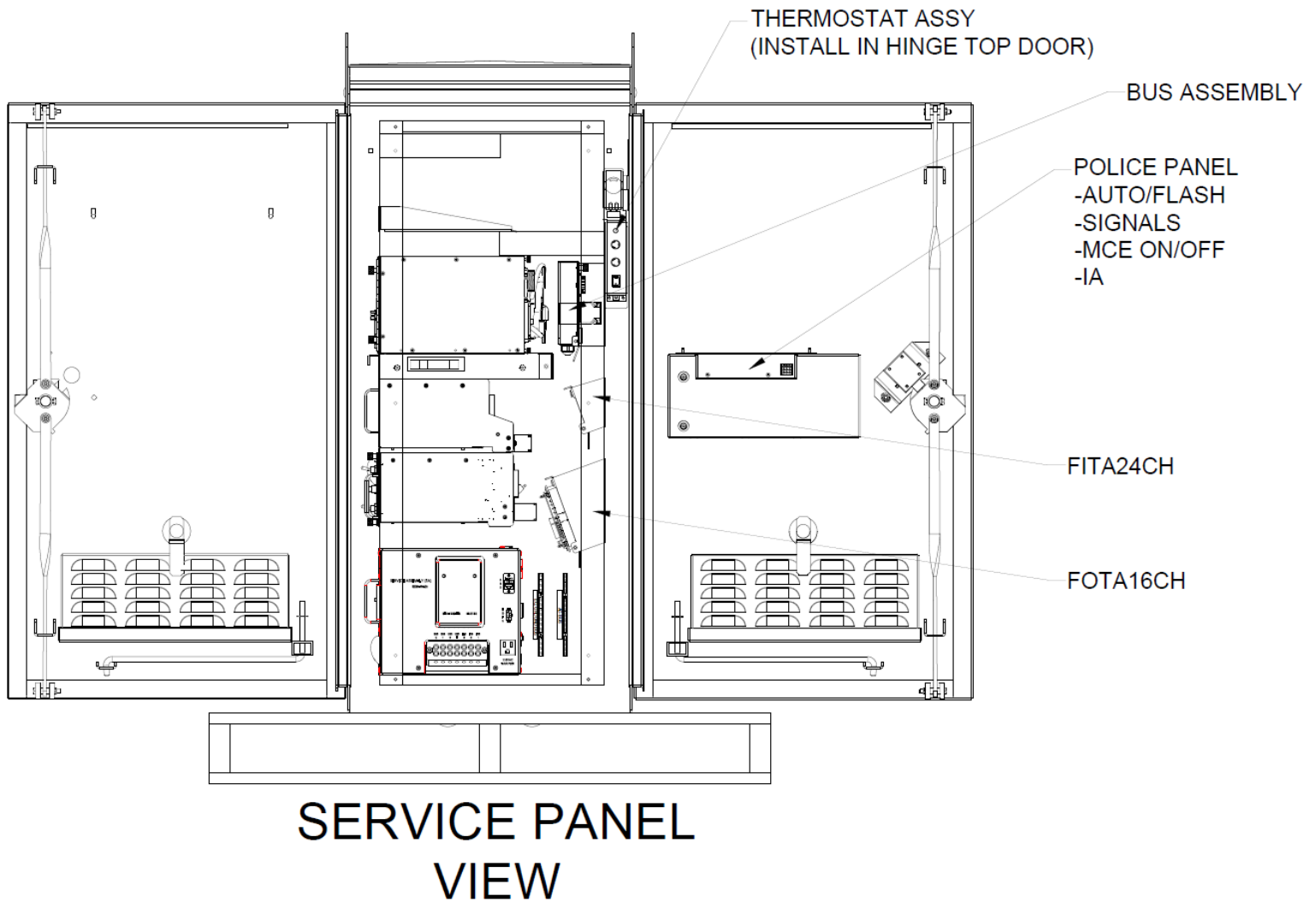
Figure 5 Cabinet Layout – ATC Cabinet 356 version (Left Side)
