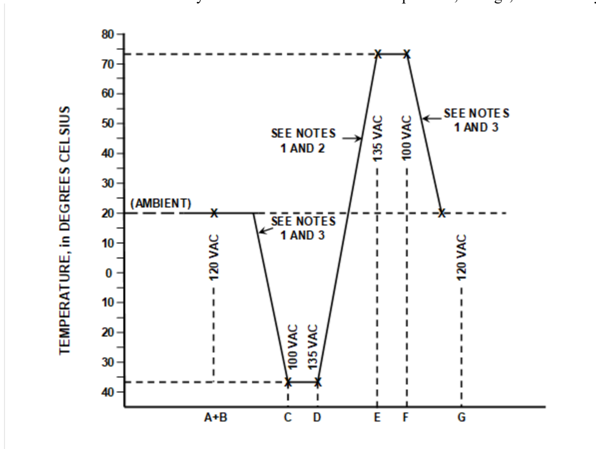
Figure 2 Test Profile
