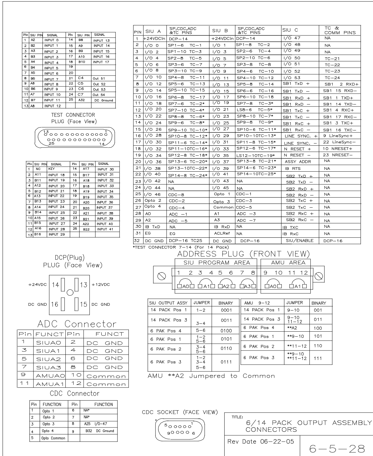
Figure 57 6/14 Pack Output Assembly Connectors
