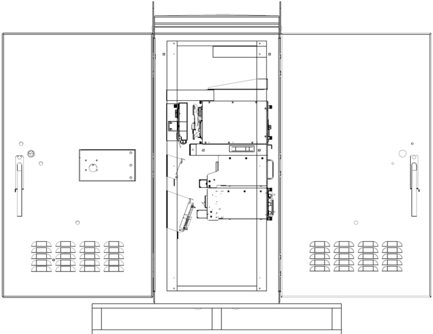
Figure 6 Cabinet Layout – ATC Cabinet 356 version (Right Side)
