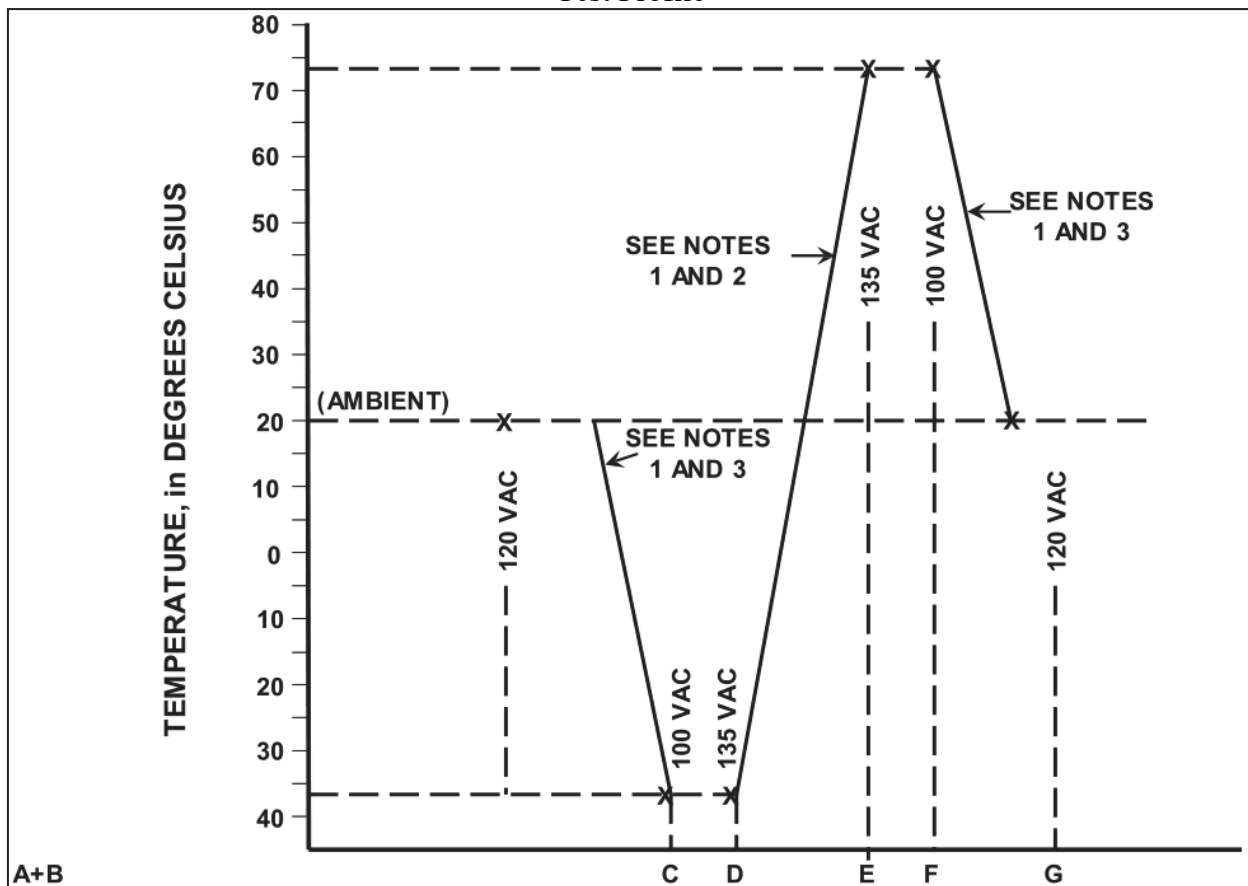
Figure 1 Test Profile
