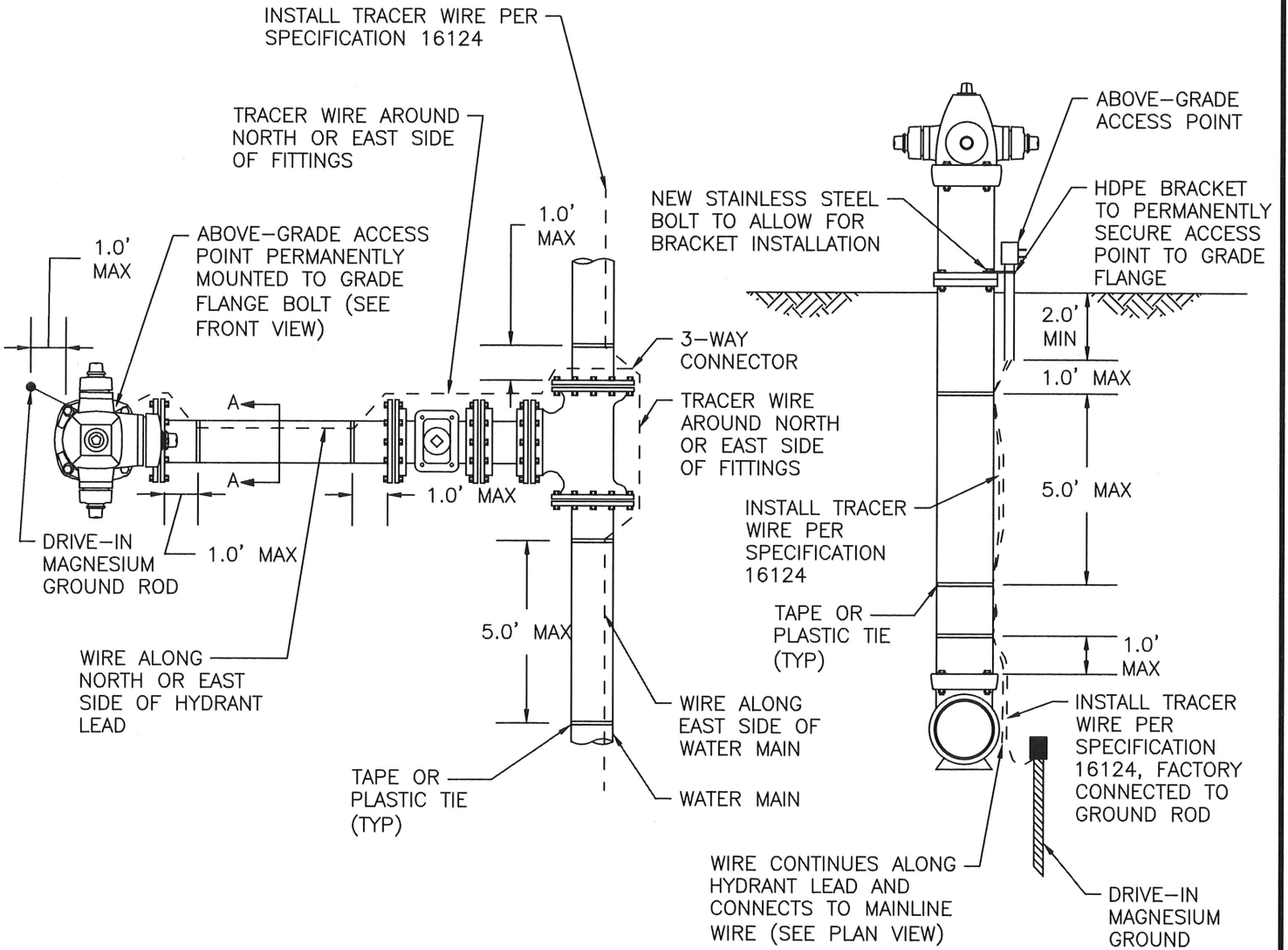
HYDRANT - PLAN VIEW NOT TO SCALE
