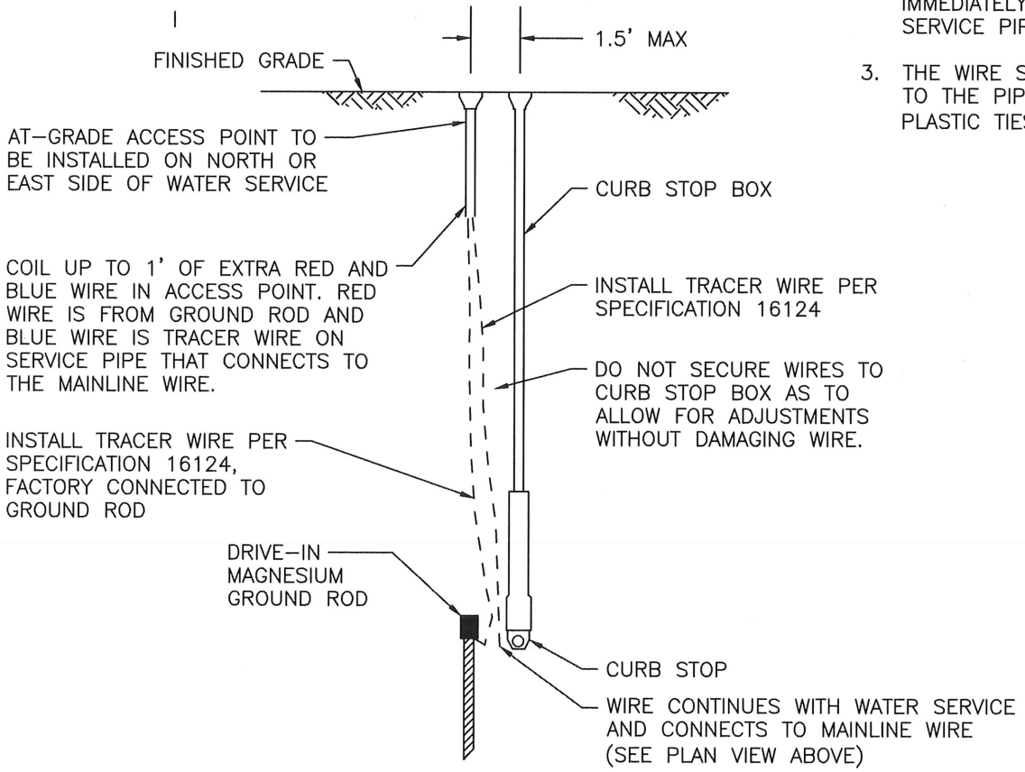
WATER SERVICE - PLAN VIEW NO SCALE
