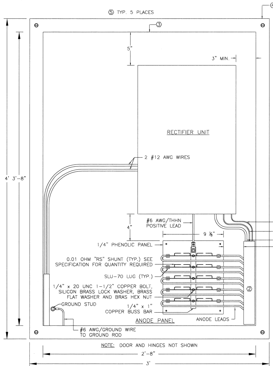
1 CATHODIC PROTECTION CABINET NO SCALE FOR O NOTES, SEE COH DETAIL 16640-03.
