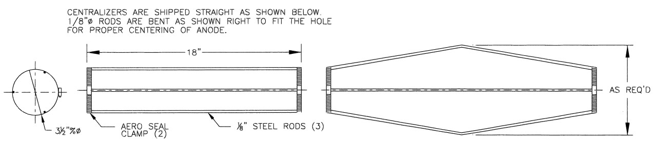
2 ANODE CENTRALIZER NO SCALE
