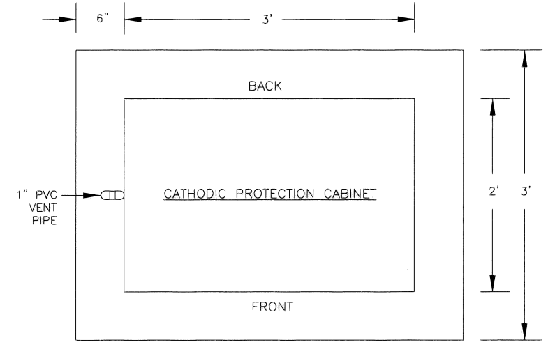
4 PLAN VIEW OF CONCRETE PAD WITH CATHODIC PROTECTION CABINET NO SCALE
