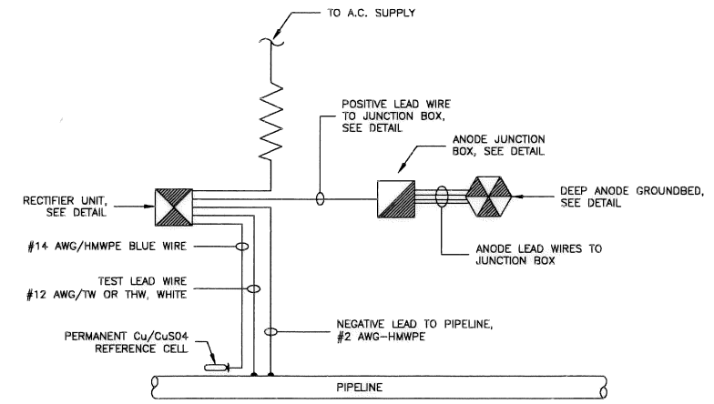
3 ELECTRICAL DIAGRAM SCHEMATIC FOR IMPRESSED CURRENT CATHODIC PROTECTION SYSTEM NOT TO SCALE
