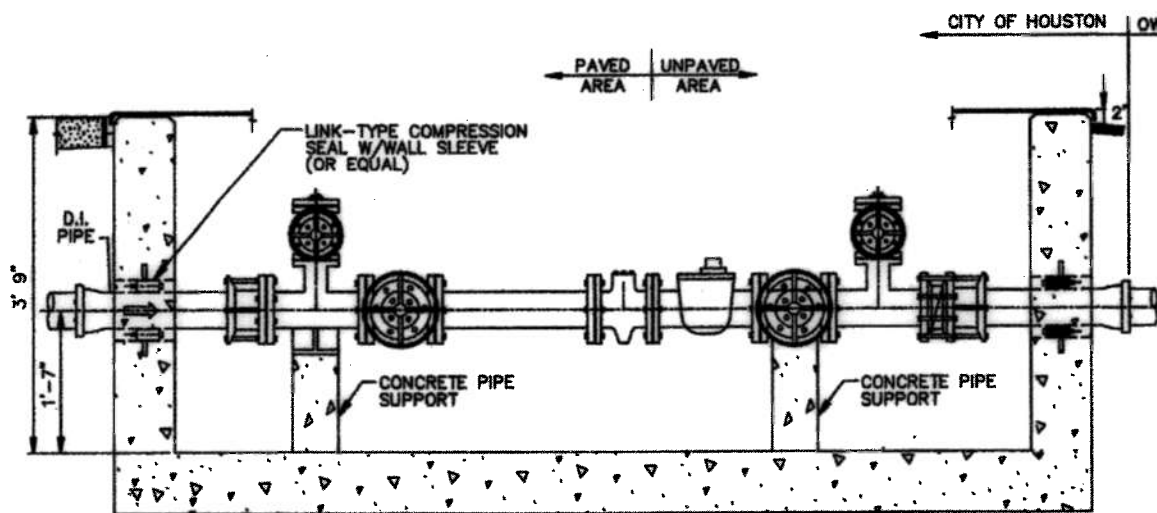
4" TURBINE METER ELEVATION VIEW
