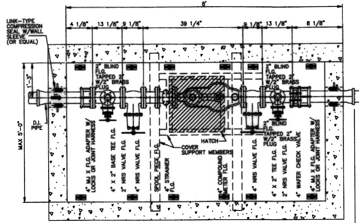
4" COMPOUND METER PLAN VIEW
