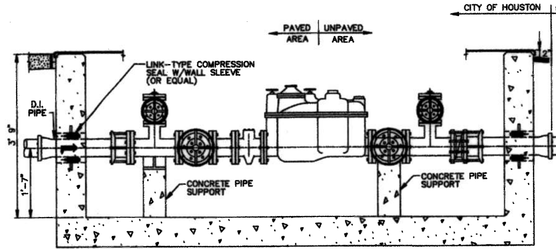
4" COMPOUND METER ELEVATION VIEW
