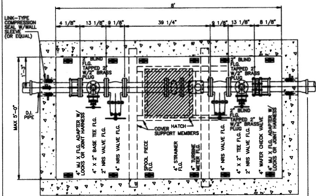
4" TURBINE METER PLAN VIEW
