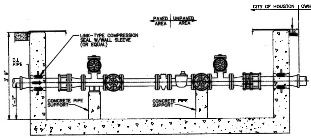
3" TURBINE METER ELEVATION VIEW
