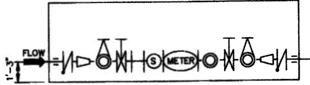
ALTERNATE PLAN VIEW (SEE NOTE 3 ON COVER PLATE PLAN)
