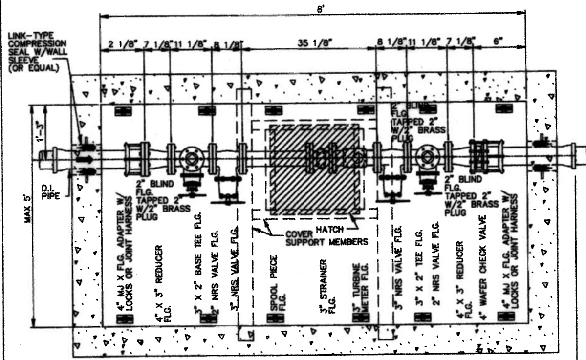
3" TURBINE METER PLAN VIEW
