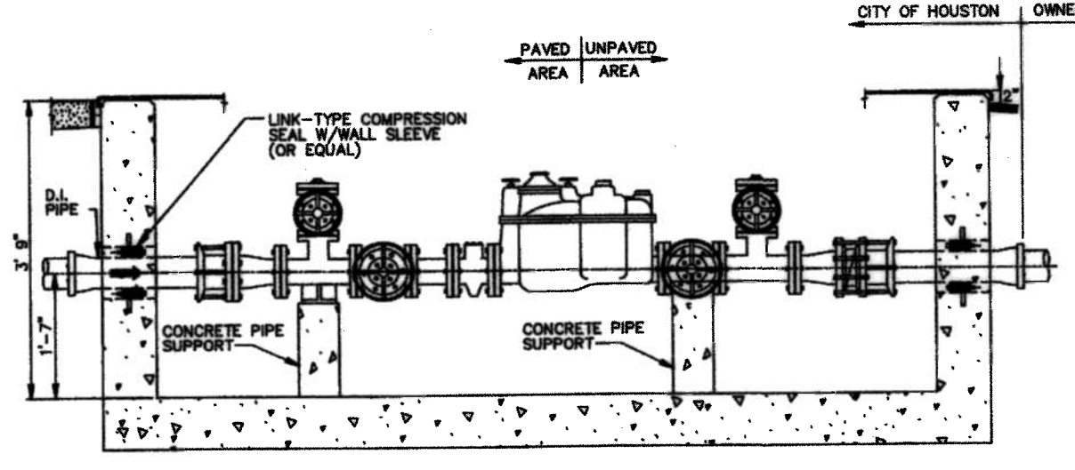
3" COMPOUND METER ELEVATION VIEW
