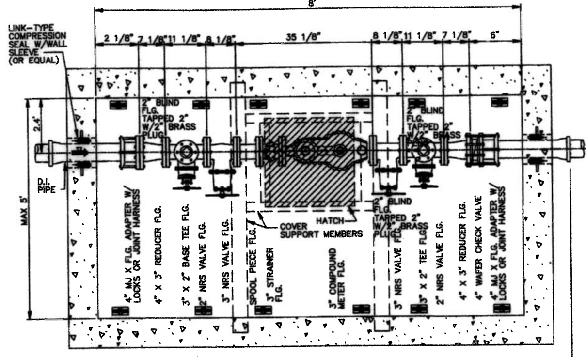
3" COMPOUND METER PLAN VIEW
