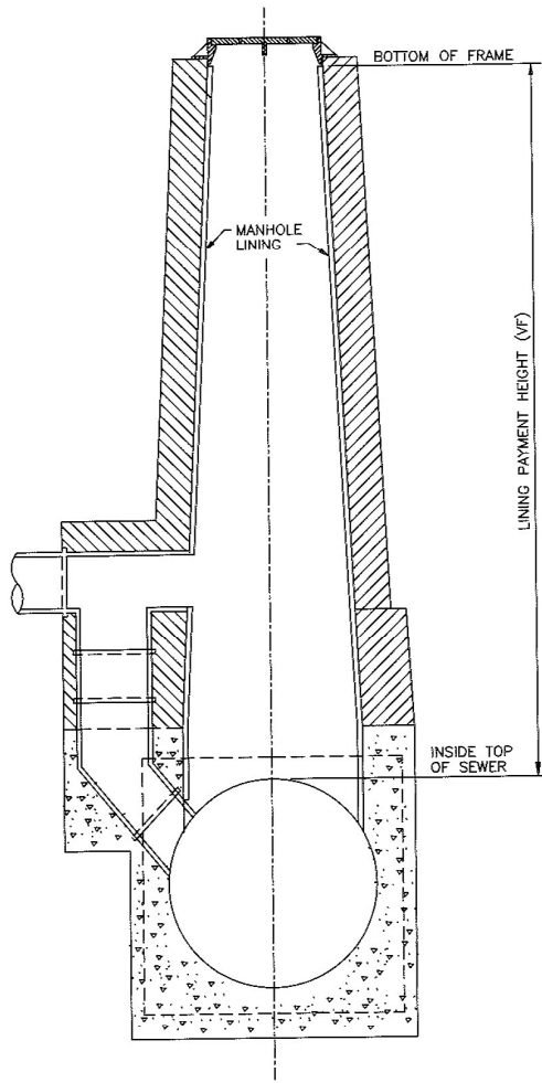
TYPICAL MONOLITHIC SEWER MANHOLE
