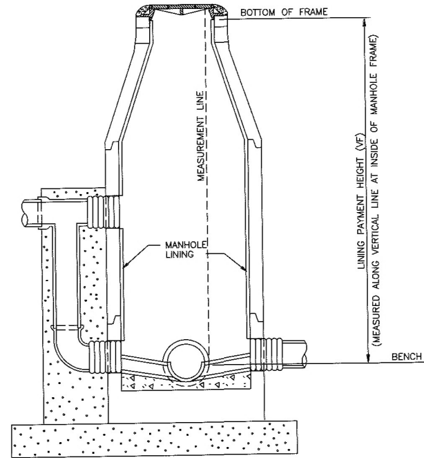
TYPICAL PIPE SEWER MANHOLE
