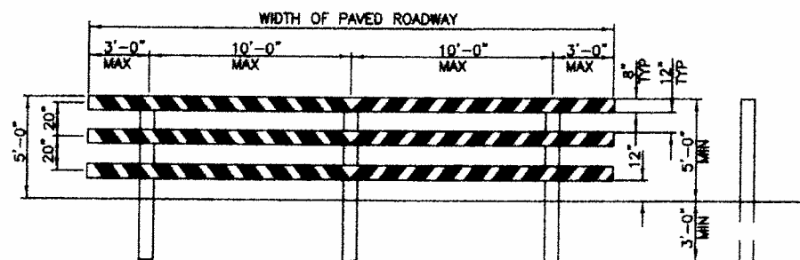
TYPE III BARRICADE FOR END OF ROAD
