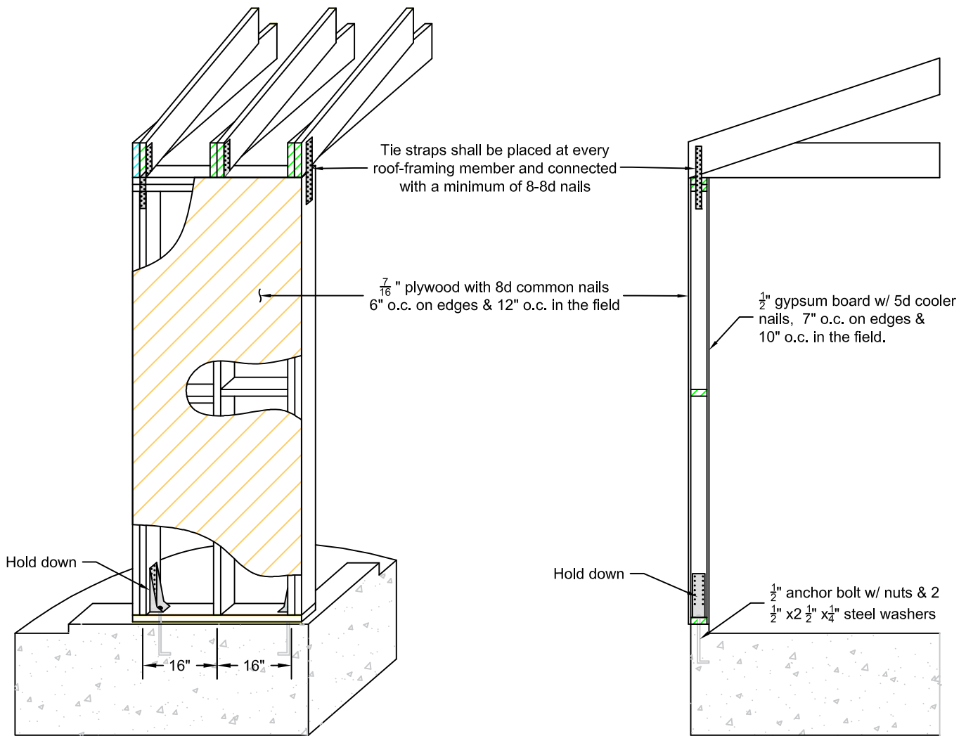
SHEAR WALL SEGMENT
